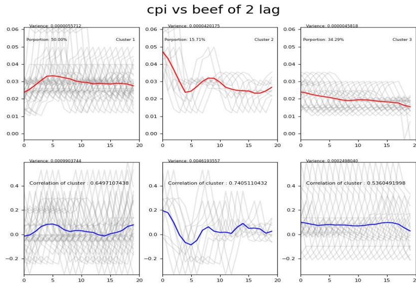
Figure 3. CPI as the explanatory variable, and beef price as the response variable. Each grey line stands for one 5-year time series t . Top row: CPI is clustered into three groups. Bottom row: the corresponding beef price curves with lag=2 (six months delay). Red line for the average curve of CPI. Blue line for the average curve of beef.
