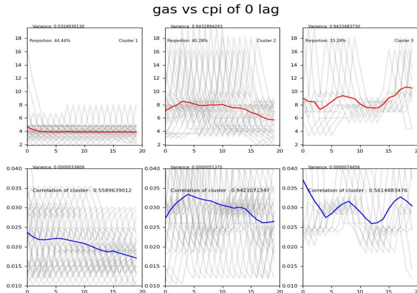
Figure 4. Gas price as the explanatory variable, and CPI as the response variable. Top row: Gas price clustered into three groups. Bottom row: the corresponding CPI with lag=0 (no delay). Red line for the average curve of gas price. Blue line for the average curve of CPI.
