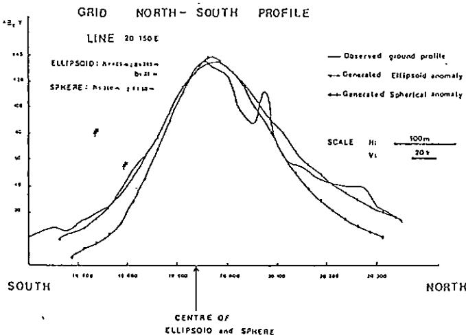
FIGURE 2 Comparison of observed ground magnetic anomaly with theoretical anomalies for ellipsoid and sphere models.
