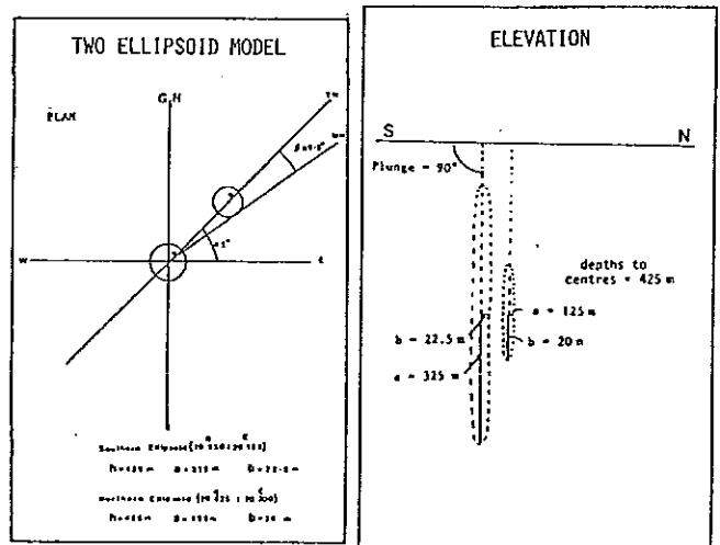
FIGURE 4 Geometry of two-ellipsoid model of Elura orebody.
