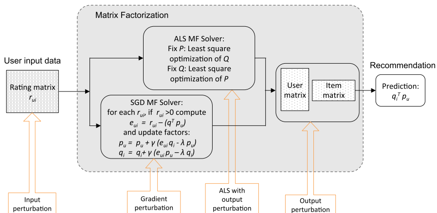
Fig. 1 Different noise application points in regards to the input, output and the solver within the matrix factorization mechanism
