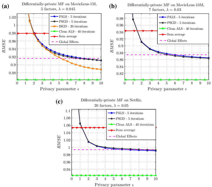
Fig. 4 Unbounded differentially-private matrix factorization. a MovieLens-1M. b MovieLens-10M. c Netflix
