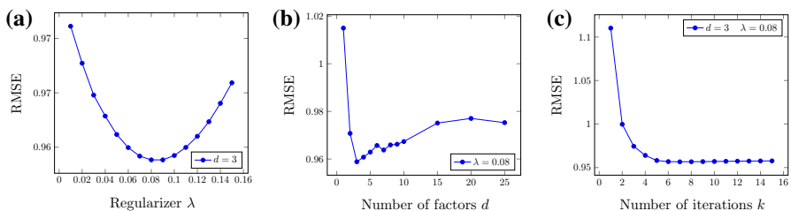
Fig. 6 Parameterization of the differentially-private matrix factorization. a Setting \lambda . b Setting d . c Setting k
