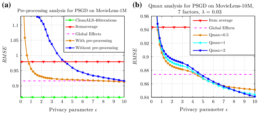
Fig. 3 Impact of preprocessing and bounding. a The impact of data preprocessing. b The impact of factor vector L_2 -norm bounds
