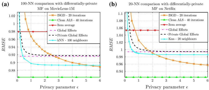
Fig. 5 Private matrix factorization and kNN comparisons. a Private kNN on MovieLens-1M. b Private kNN on Netflix
