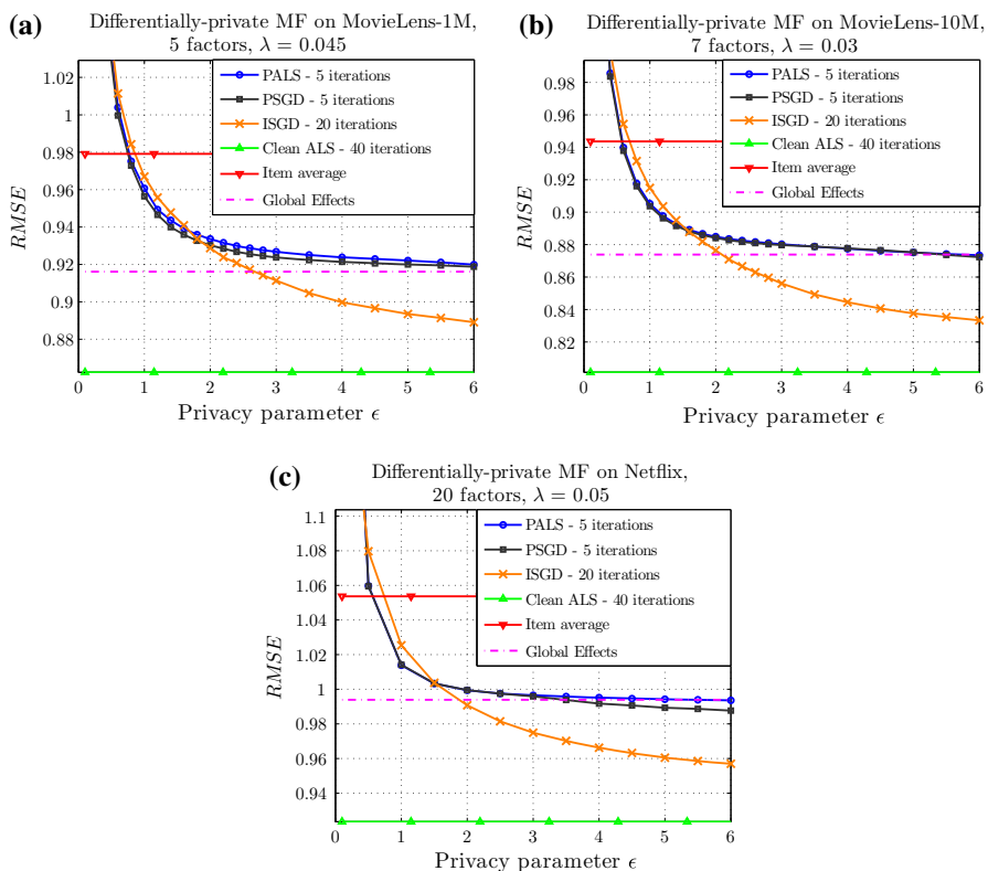
Fig. 2 Bounded differentially-private matrix factorization. a MovieLens-1M. b MovieLens-10M. c Netflix
