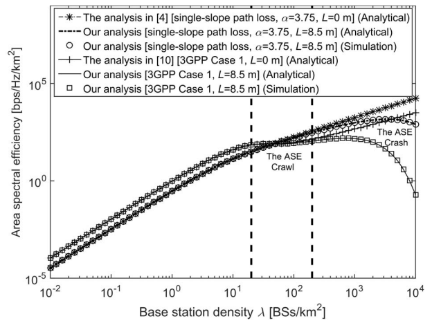
Fig. 4. A^{\text{ASE}}(\lambda, \gamma_0) vs. \lambda with \gamma_0 = 0 dB.
