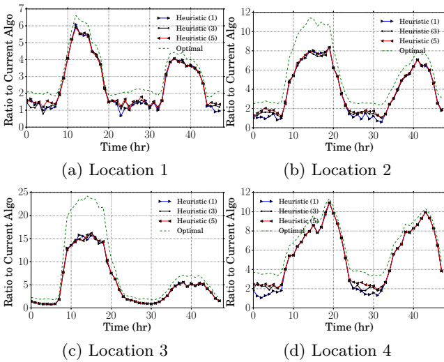
Figure 10: Heuristic Performance
