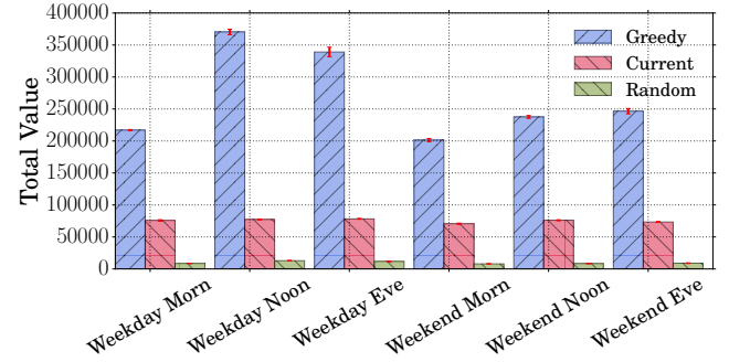
Figure 7: Temporal performance variation
