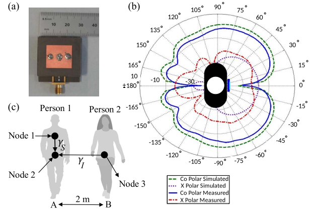
Fig. 3. (a) HMPA. (b) Simulated far-field radiation patterns of HMPA in azimuth plane at 2.484 GHz when placed on a human tissue phantom. (c) Position of BAN nodes. On-body transmitter located on front-chest of person 1 (Node 1) and front-central-waist of person 2 (Node 3). Receiver positioned on the front-central-waist of person 1 (Node 2). SoI operated between Nodes 1 and 2, while the interfering signal operated between Nodes 3 and 2. A and B denote the positions of the test subjects in each of the environments.
