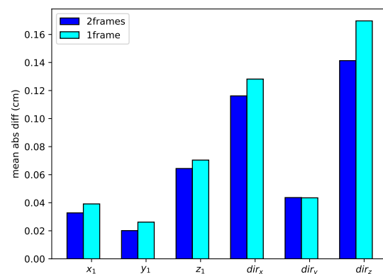
Fig. 4: Comparison between the network when it trained with a pair of consecutive frames versus one frame to estimate CCL parameters, here (x_1, y_1, z_1) represent centerline point and dir is for the direction of colon centerline.
