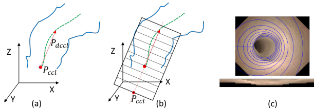
Fig. 2: (a) A colon with its centerline, P_{ccl} is a point on the CCL and P_{dcccl} is the direction to a second point (red arrow), (b) a cylinder generated in the direction of colon and (c) is the projection of cylinder onto the image and the band image.
