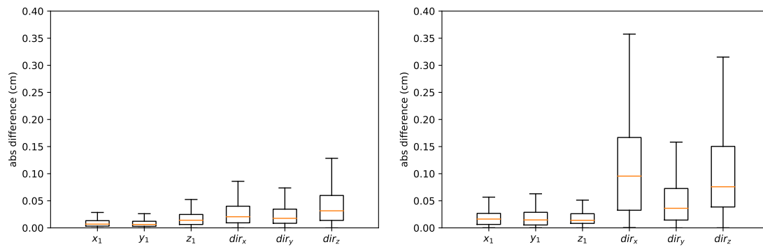
Fig. 3: Validation of trained VGG on simulated training dataset (left panel), Test network for generalization by using a simulated colonoscopy video which has not been used in training or validation (right panel). x , y , z represents centerline point and dir is for the direction of colon.
