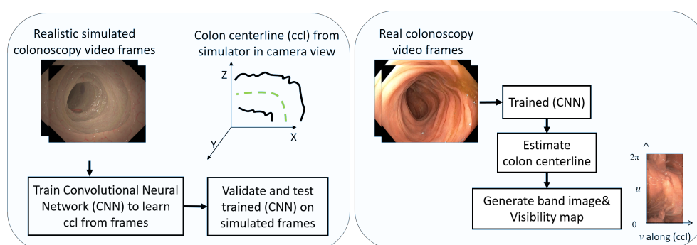
Fig. 1: A schematic of the proposed processing pipeline.
