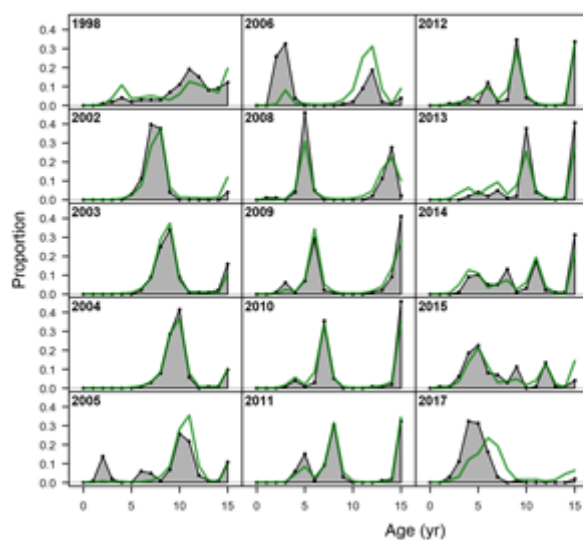
Figure A 10.13. Age composition fits: spawning fleet onboard retained.
