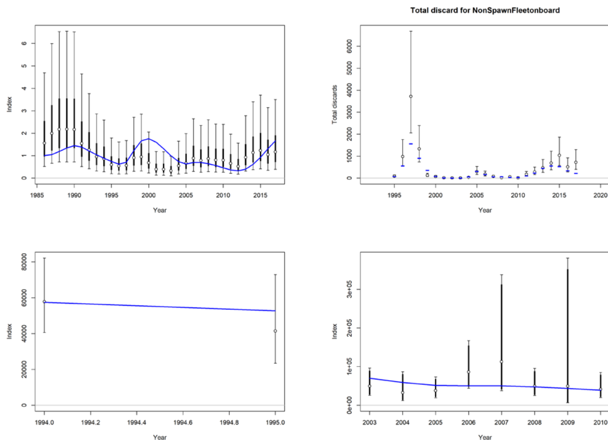
Figure A 10.4. Fits to the non-spawning CPUE index, discard mass, egg survey and acoustic survey.
