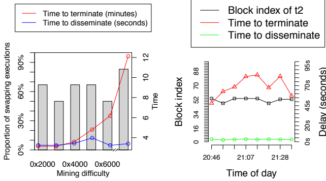
(a) The proportion of transaction swaps observed does not depend on Blockchain anomalies over a period of 50 min, as opposed to the non-sensus termination that increases with the difficulty (b) Automated executions of the anomaly are deterministic due to the randomness of the mining process and the network delay between peers
