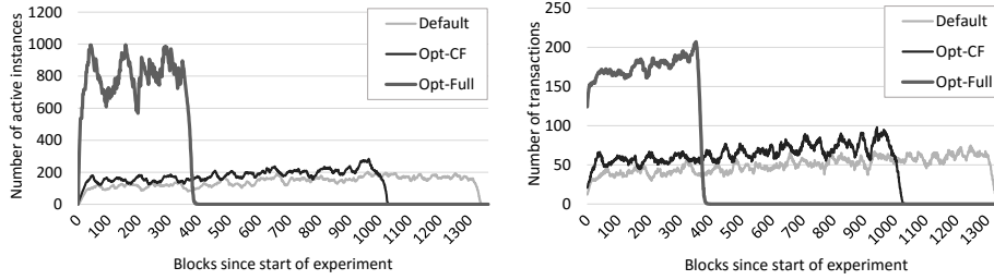
Fig. 7: Throughput results. Left: # of active instances. Right: # of transactions per block, smoothed over a 20-block time window.
