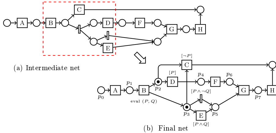
Fig. 6: Reduced Petri net corresponding to the BPMN model in Fig. 2
