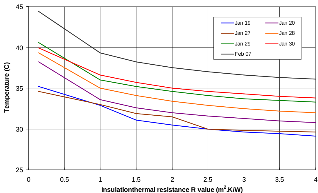
Figure 4.7: Changes of daily maximum temperature in Bedroom 1 with R values on days hotter than 35°C
