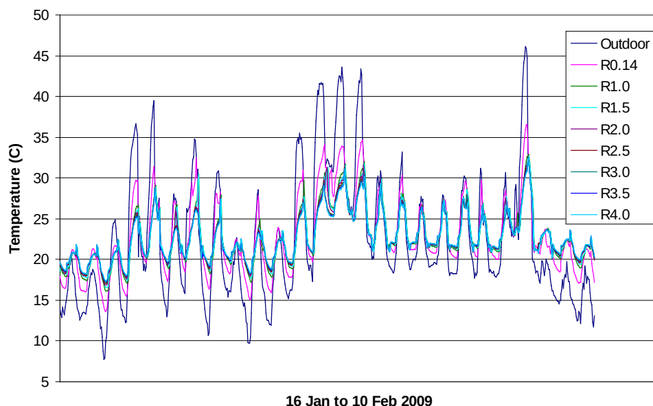
Figure 4.5: Changes of temperature in Bedroom 1 with time at different R values
