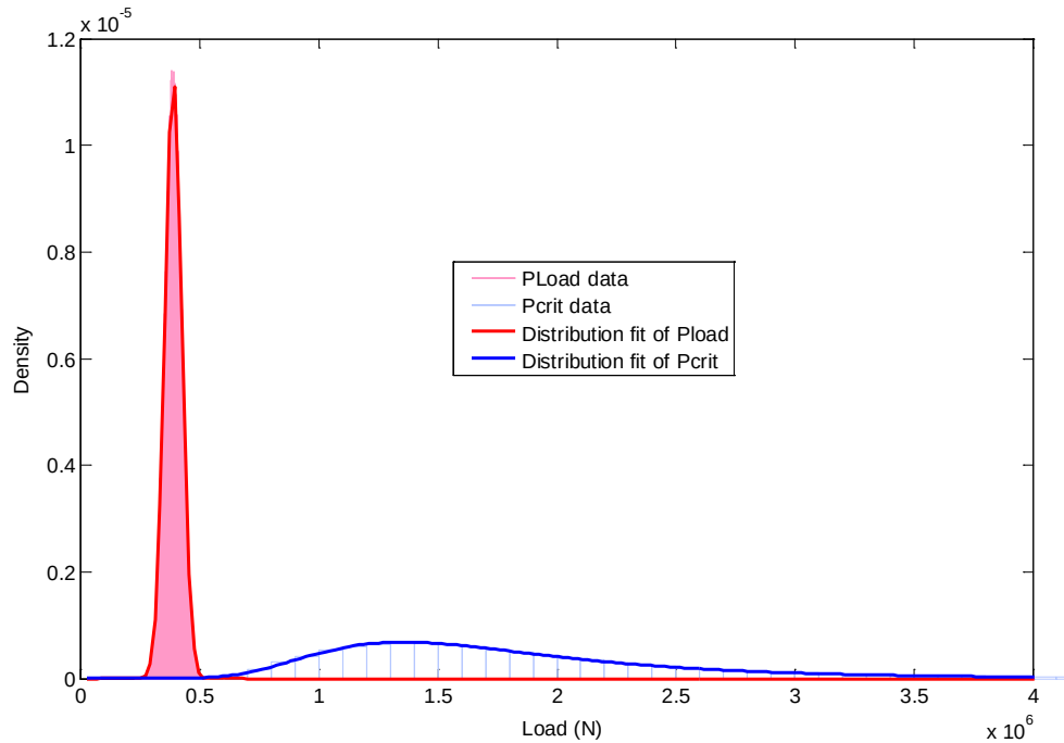
Figure 4.10: Distributions of thermal loads and critical loads estimated for Melbourne railways due to January 2009 heatwave in Melbourne
