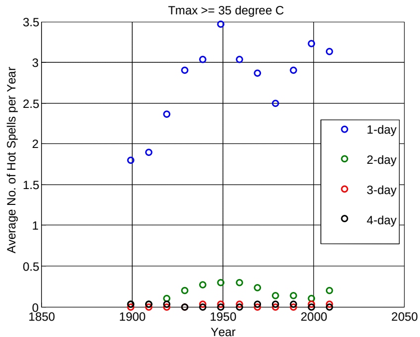
Figure F.2.3: Changes in the yearly number of 1-day, 2-day, 3-day, and 4-day hot spells with T_{max} \geq 35^{\circ}\text{C} – Sydney Observatory Hill station
