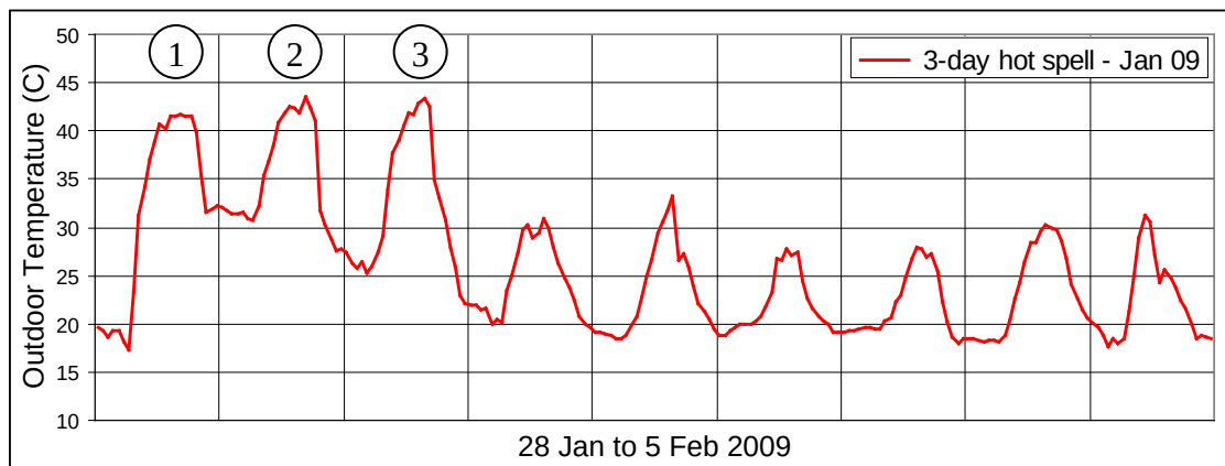
Figure 4.2: Scenario 1: Temperature record from 28 January to 5 February 2009
