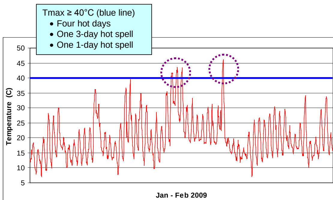
Figure 1.1: Hourly temperature between January and February 2009 showing four days with T_{max} \geq 40^{\circ}\text{C} . The purple circles illustrate a 3-day hot spell and a 1-day hot spell with T_{max} \geq 40^{\circ}\text{C} .
