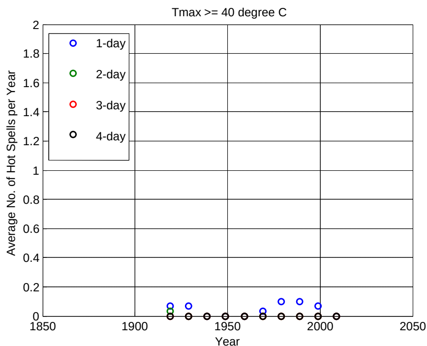
Figure F.1.4: Changes in the yearly number of 1-day, 2-day, 3-day, and 4-day hot spells with T_{max} \geq 40^{\circ}\text{C} – Hobart Ellerslie Rd station
