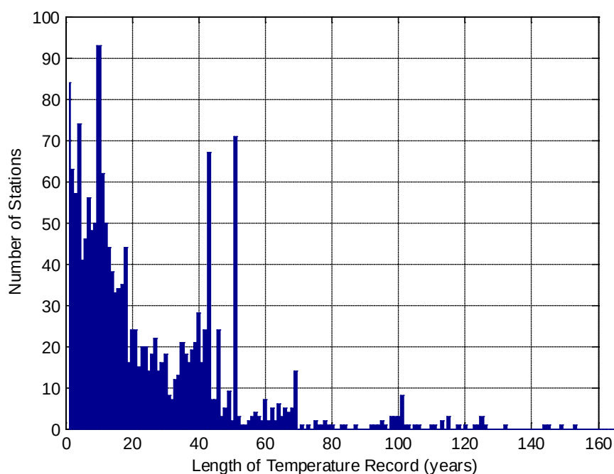
Figure 1.3: Temperature record length versus number of stations
