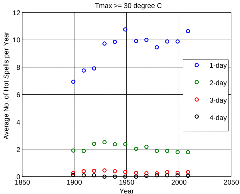
Figure F.2.2: Changes in the yearly number of 1-day, 2-day, 3-day, and 4-day hot spells with T_{max} \geq 30^{\circ}\text{C} – Sydney Observatory Hill station
