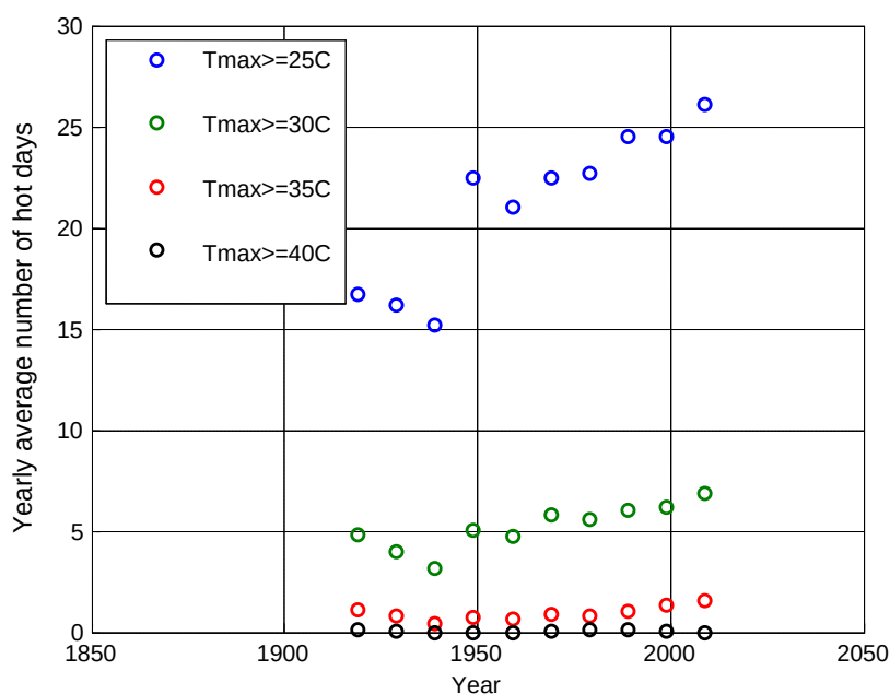
Figure F.1.1: Changes observed in the yearly number of hot days - Hobart Ellerslie Rd station
