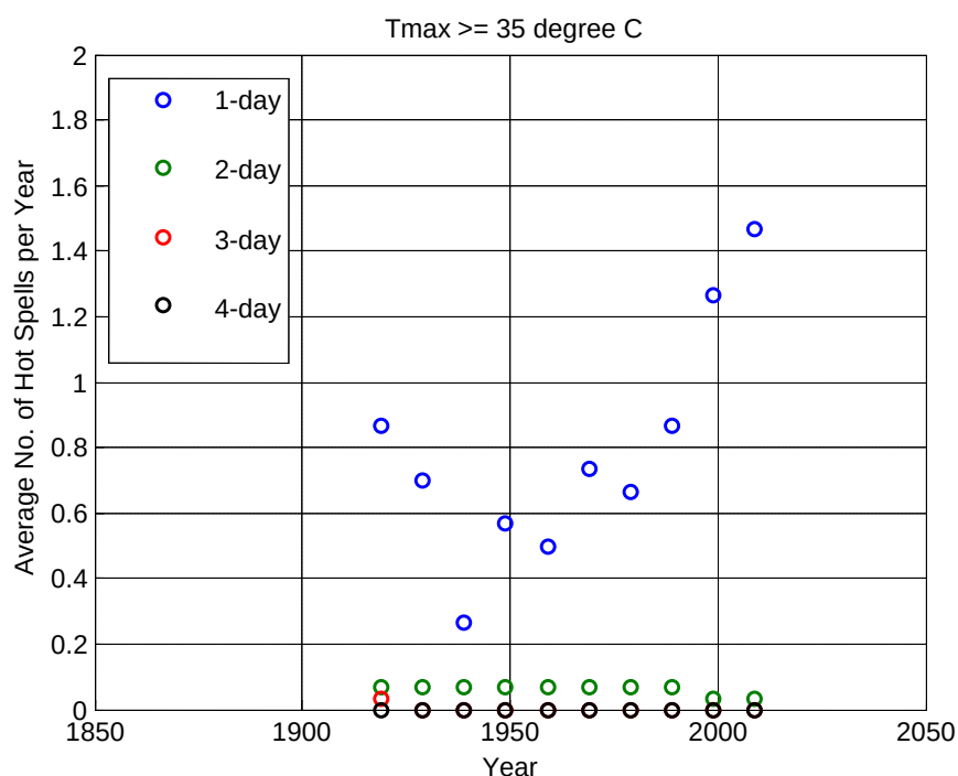
Figure F.1.3: Changes in the yearly number of 1-day, 2-day, 3-day, and 4-day hot spells with T_{max} \geq 35^{\circ}\text{C} – Hobart Ellerslie Rd station
