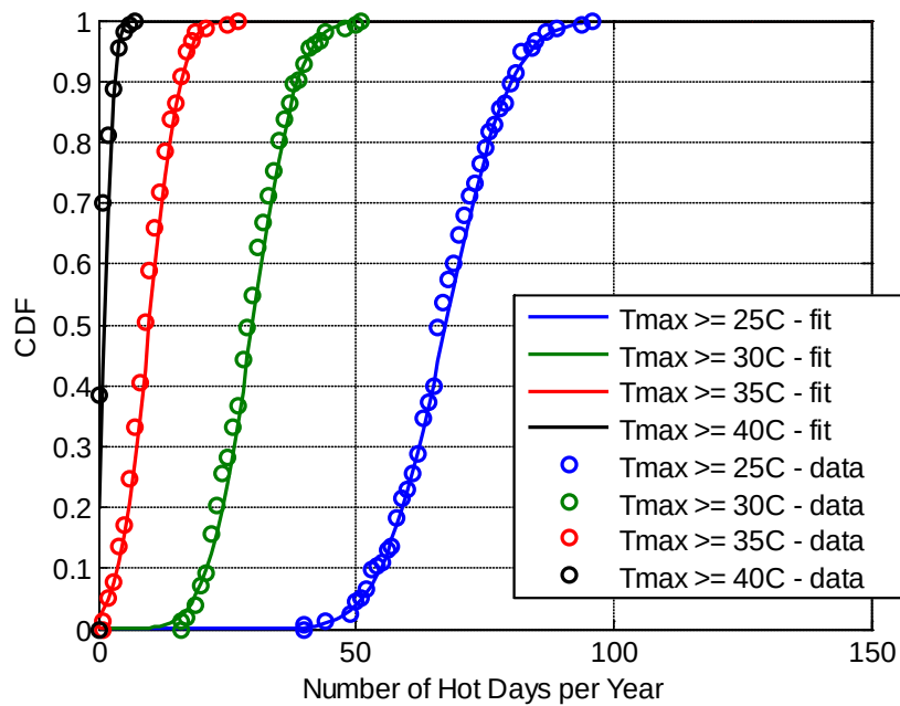
Figure 2.2: CDF of yearly number of hot days - Melbourne Regional Office Station
