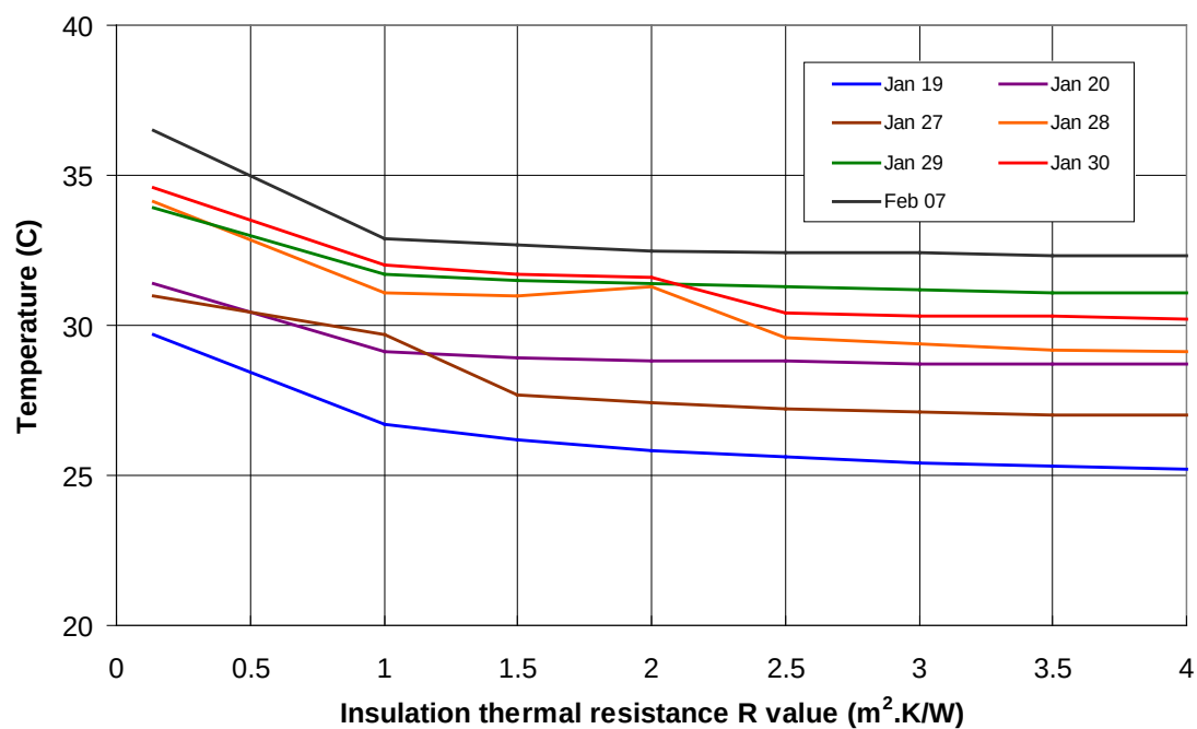
Figure 4.8: Changes of daily maximum temperature in Kitchen-Family room with R values on days hotter than 35°C
