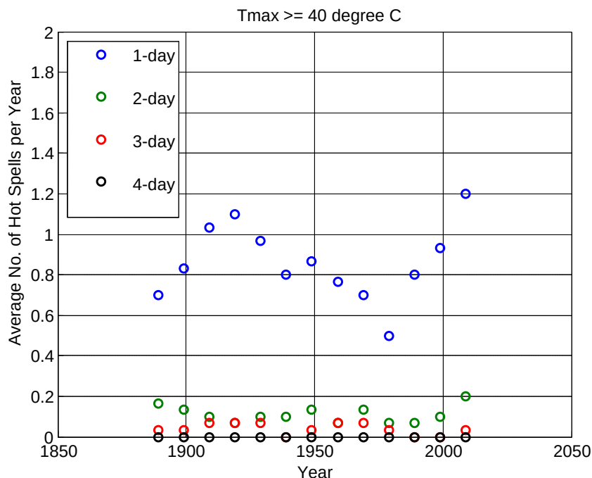
Figure 3.4: Changes in the yearly individual number of 1-day, 2-day, 3-day, and 4-day hot spells with T_{\max} \geq 40^{\circ}\text{C} – Melbourne Regional Office station
