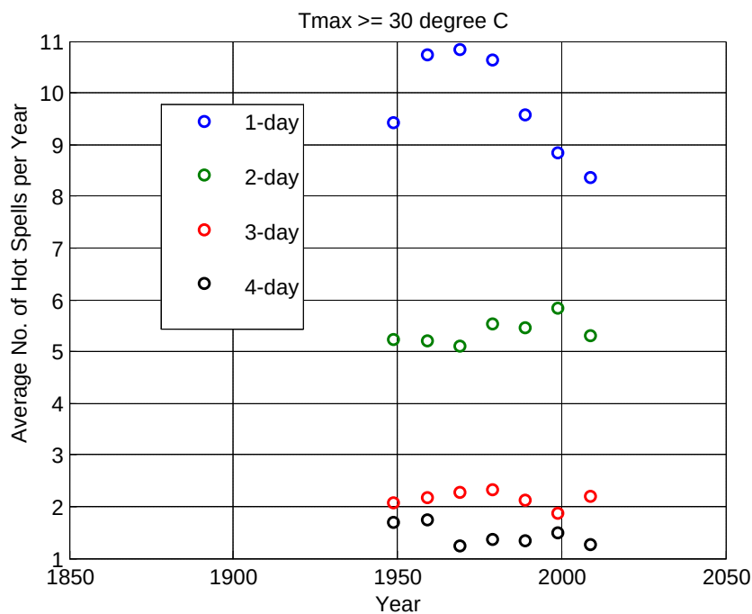
Figure F.4.2: Changes in the yearly number of 1-day, 2-day, 3-day, and 4-day hot spells with T_{max} \geq 30^{\circ}\text{C} – Adelaide West Terrace station
