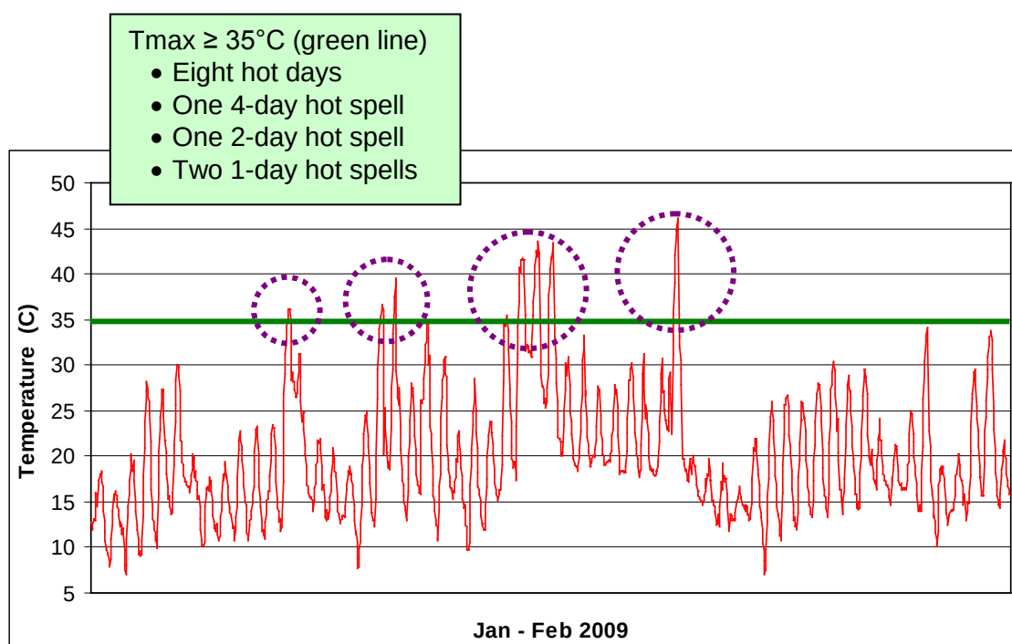
Figure 1.2: Hourly temperature between January and February 2009 showing 8 days with T_{max} \geq 35^{\circ}\text{C} . The purple circles illustrate a 4-day hot spell, a 2-day hot spell and two 1-day hot spell with T_{max} \geq 35^{\circ}\text{C} .
