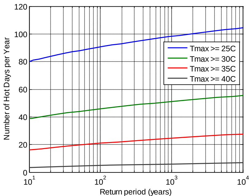
Figure 2.3: Return period of yearly number of hot days with different maximum temperature thresholds
