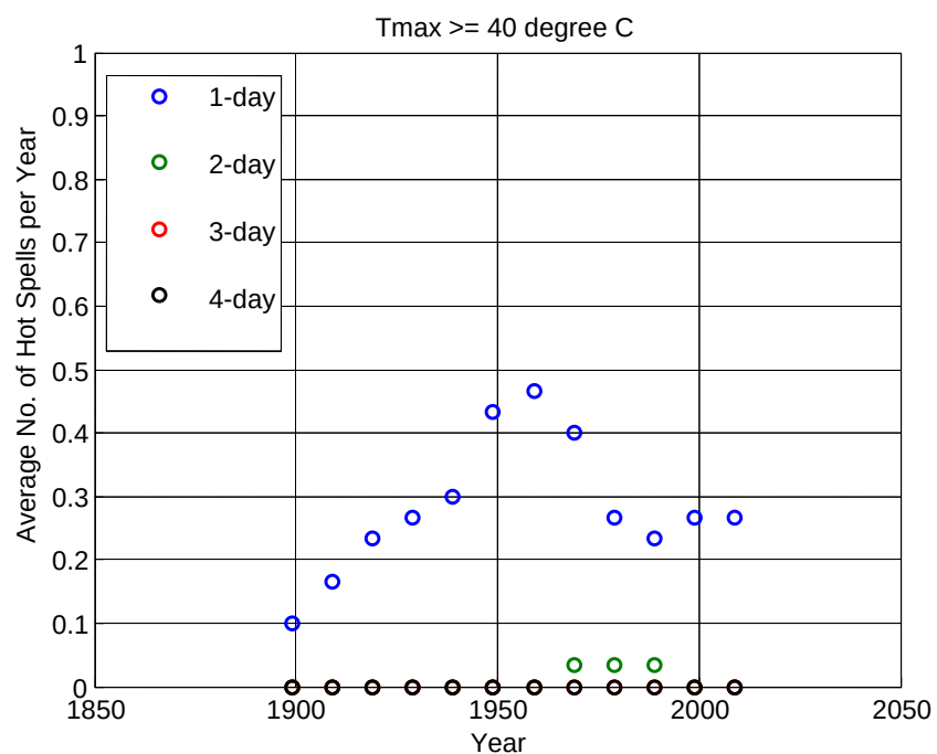
Figure F.2.4: Changes in the yearly number of 1-day, 2-day, 3-day, and 4-day hot spells with T_{max} \geq 40^{\circ}\text{C} – Sydney Observatory Hill station
