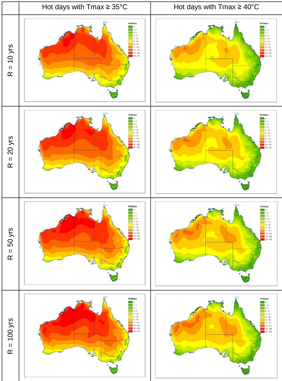
Figure 2.4: Contour maps of the frequency of number of hot days with maximum temperature threshold of 35^{\circ}\text{C} and 40^{\circ}\text{C} at different return periods
