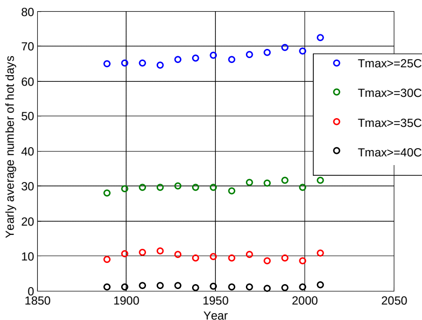
Figure 3.1: Changes observed in the yearly number of hot days - Melbourne Regional Office station
