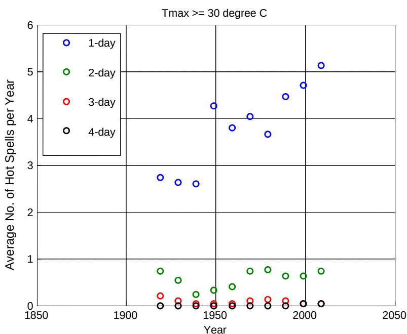
Figure F.1.1: Changes observed in the yearly number of hot days - Hobart Ellerslie Rd station
