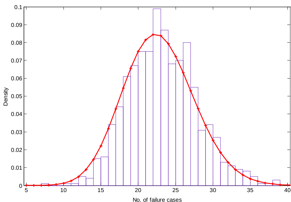
Figure 4.11: Distributions of the number of failure cases in 1000 times repeating the Monte-Carlo simulation
