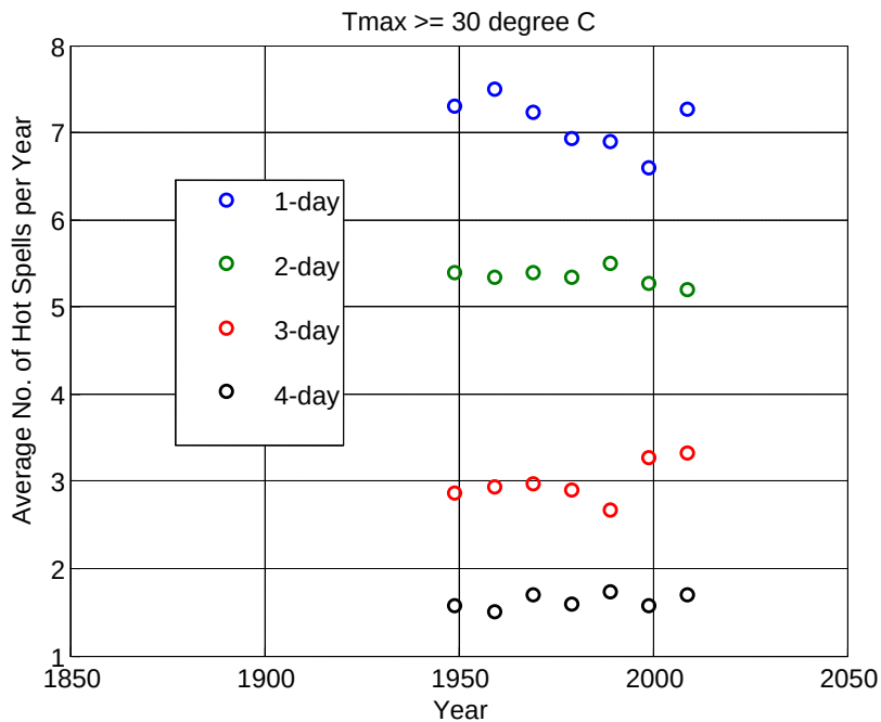
Figure F.5.2: Changes in the yearly number of 1-day, 2-day, 3-day, and 4-day hot spells with T_{max} \geq 30^{\circ}\text{C} – Perth Regional Office station
