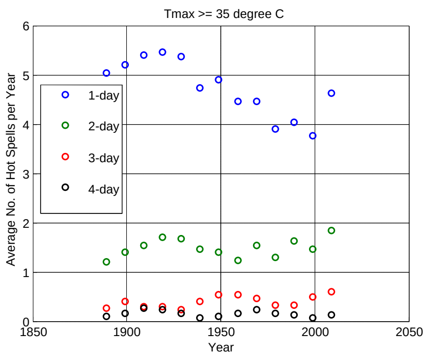
Figure 3.3: Changes in the yearly individual number of 1-day, 2-day, 3-day, and 4-day hot spells with T_{\max} \geq 35^{\circ}\text{C} – Melbourne Regional Office station
