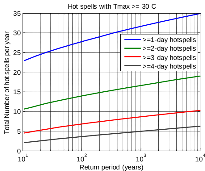
Figure 2.9: Return period versus yearly total number of hot spells with T_{max} \geq 30^\circ\text{C} – Melbourne Regional Office Station
