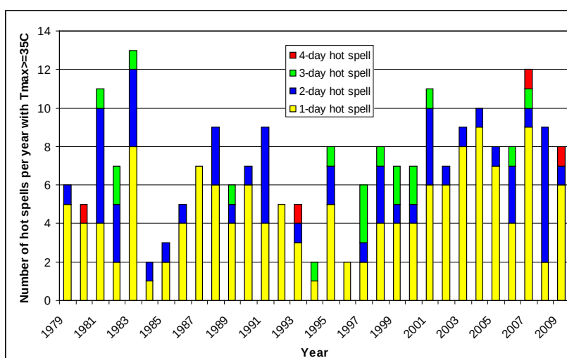
Figure 2.5: Yearly number of 1-day, 2-day, 3-day, and 4-day hot spells with threshold temperature of 35°C at Melbourne Regional Station
