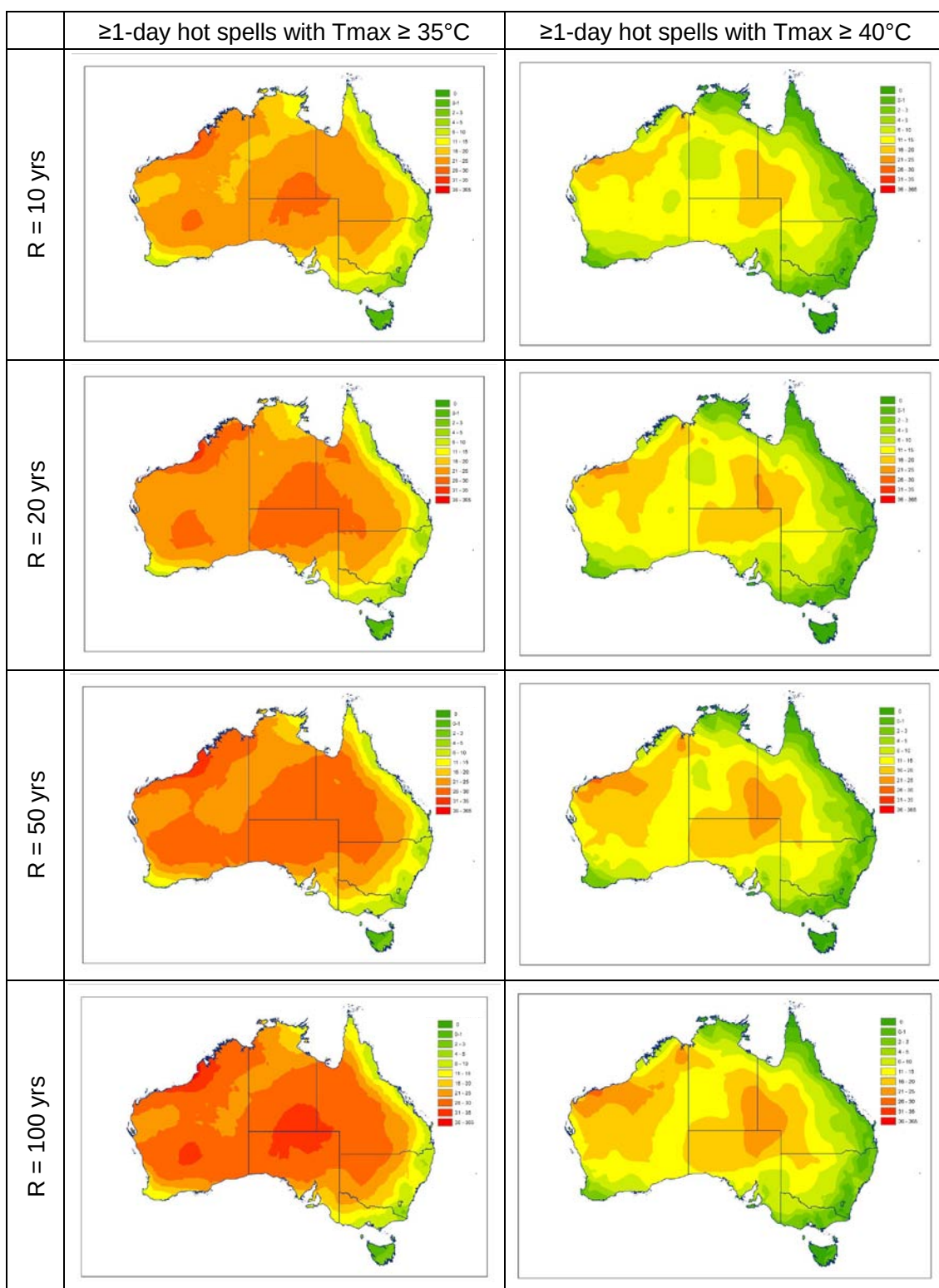
Figure 2.12: Contour map of yearly total number of hot spells that last 1 day or more with maximum temperature threshold of 35^{\circ}\text{C} and 40^{\circ}\text{C} at different return periods
