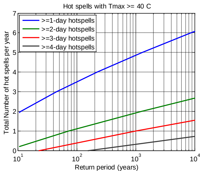
Figure 2.11: Return period versus yearly total number of hot spells with T_{max} \geq 40^\circ\text{C} – Melbourne Regional Office Station
