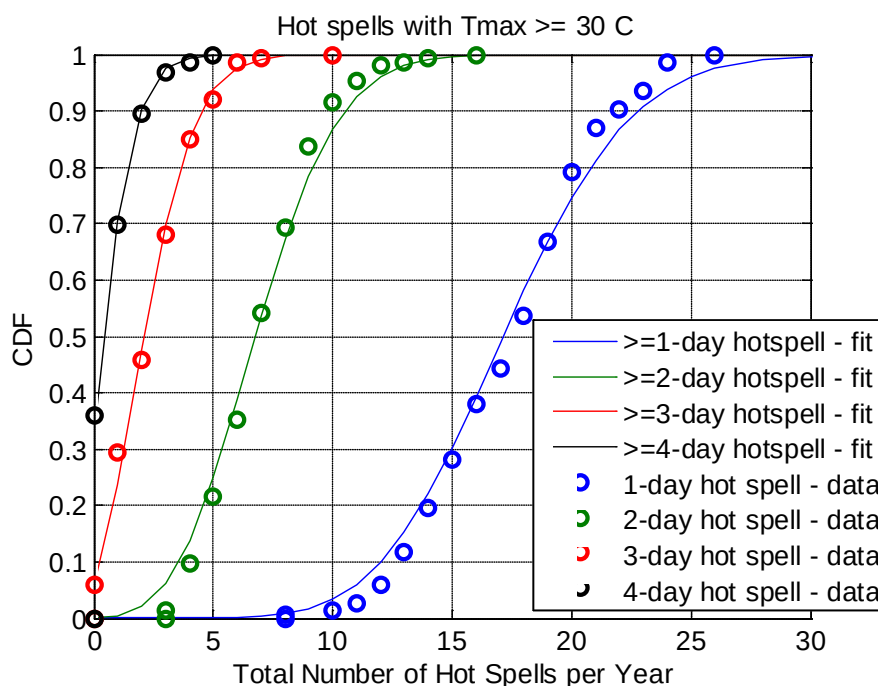
Figure 2.6: Fitting the Poisson distribution to the yearly total number of hot spells with Tmax ≥ 30°C – Melbourne Regional Office Station
