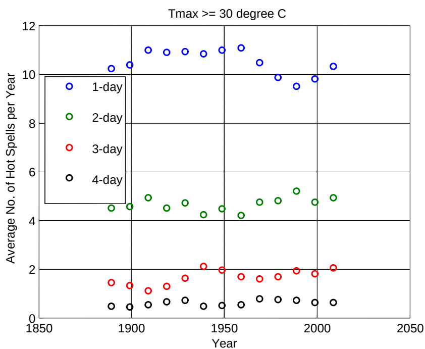
Figure 3.2: Changes in the yearly individual number of 1-day, 2-day, 3-day, and 4-day hot spells with T_{\max} \geq 30^{\circ}\text{C} – Melbourne Regional Office station
