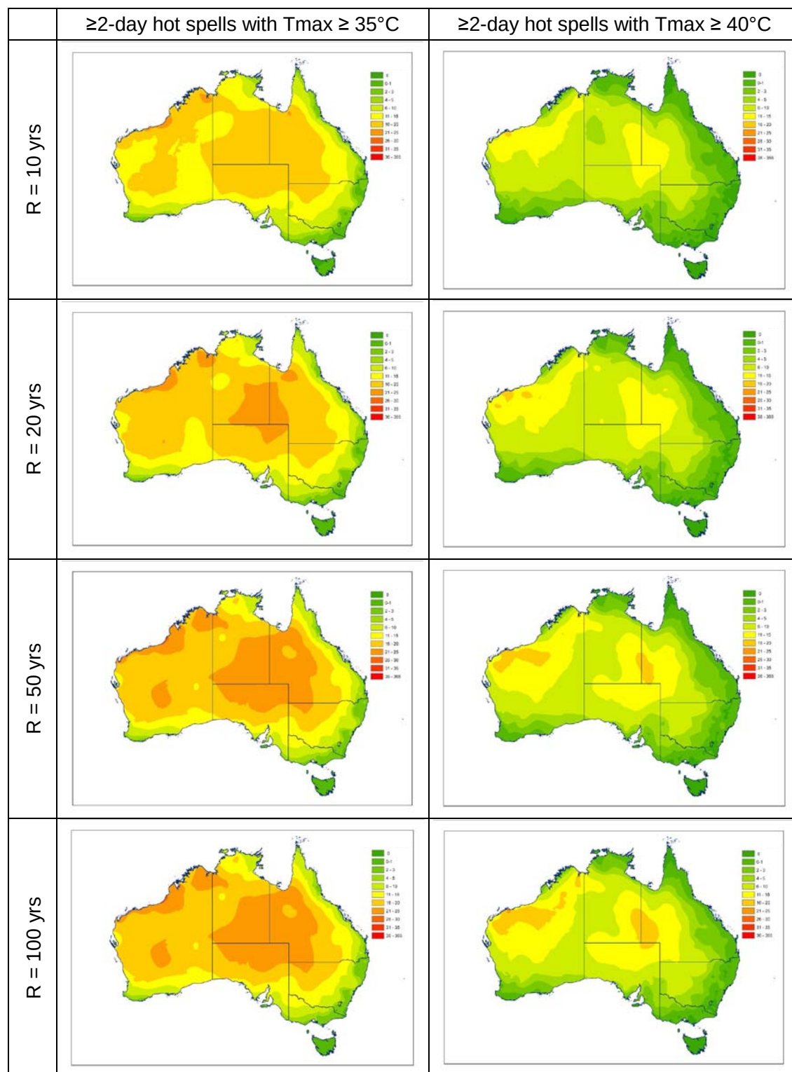
Figure 2.13: Contour map of yearly total number of hot spells that last 2 days or more with maximum temperature threshold of 35^{\circ}\text{C} and 40^{\circ}\text{C} at different return periods
