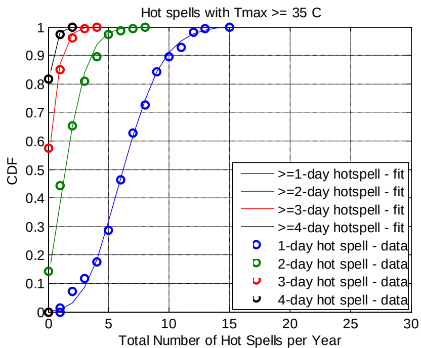
Figure 2.7: Fitting the Poisson distribution to the yearly total number of hot spells with T_{\max} \geq 35^{\circ}\text{C} – Melbourne Regional Office Station
