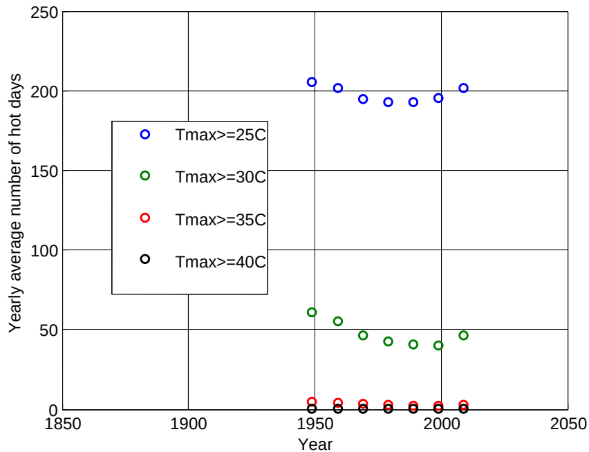
Figure F.3.1: Changes observed in the yearly number of hot days - Brisbane Regional Office
