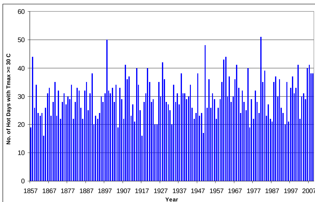
Figure 2.1: Number of hot days with T_{\max} \geq 30^{\circ}\text{C} counted every year at Melbourne Regional Station
