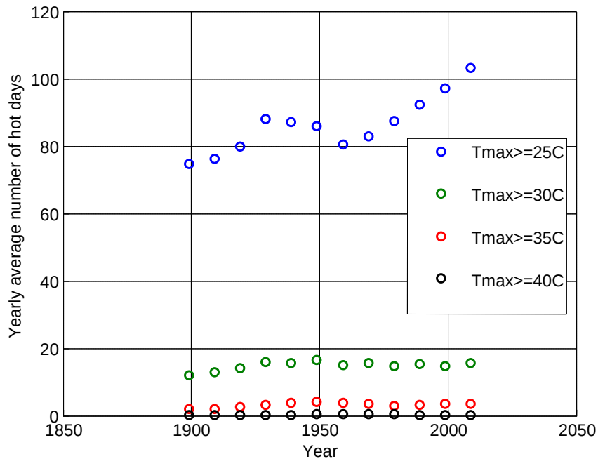
Figure F.2.1: Changes observed in the yearly number of hot days - Sydney Observatory Hill station
