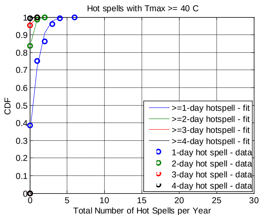
Figure 2.8: Fitting the Poisson distribution to the yearly total number of hot spells with T_{\max} \geq 40^{\circ}\text{C} – Melbourne Regional Office Station
