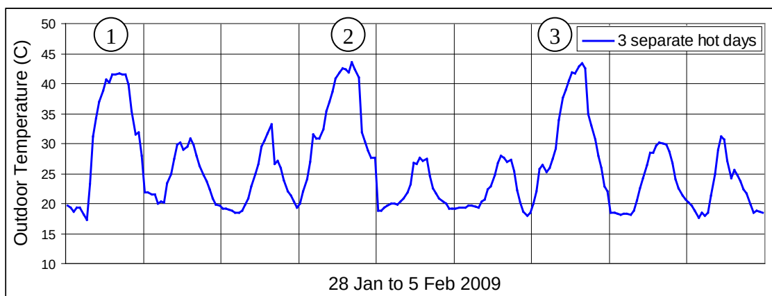
Figure 4.3: Scenario 2: Assumed temperature record from 28 January to 5 February 2009 by separating the 3-day hot spell into 3 separate hot days
