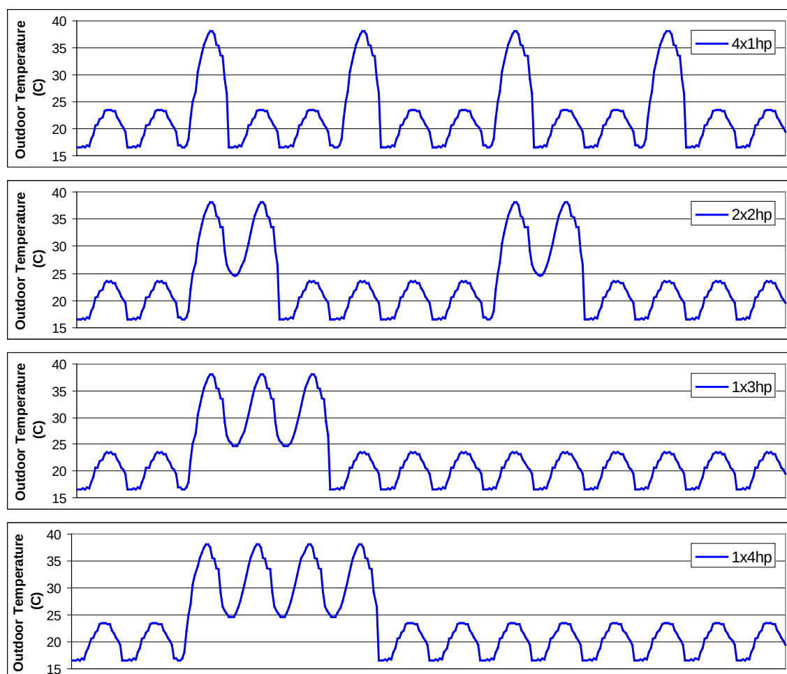
Figure 4.1: Temperature profiles for the hot spell scenarios used in this study
