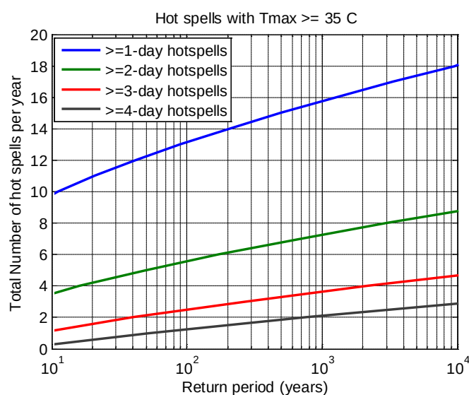
Figure 2.10: Return period versus yearly total number of hot spells with T_{max} \geq 35^\circ\text{C} – Melbourne Regional Office Station
