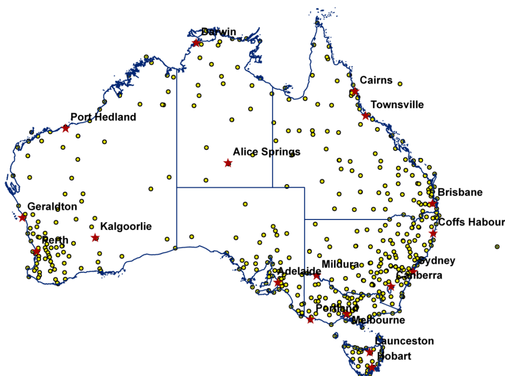
Figure 1.4: Location of 548 BOM stations having record period more than 30 years
