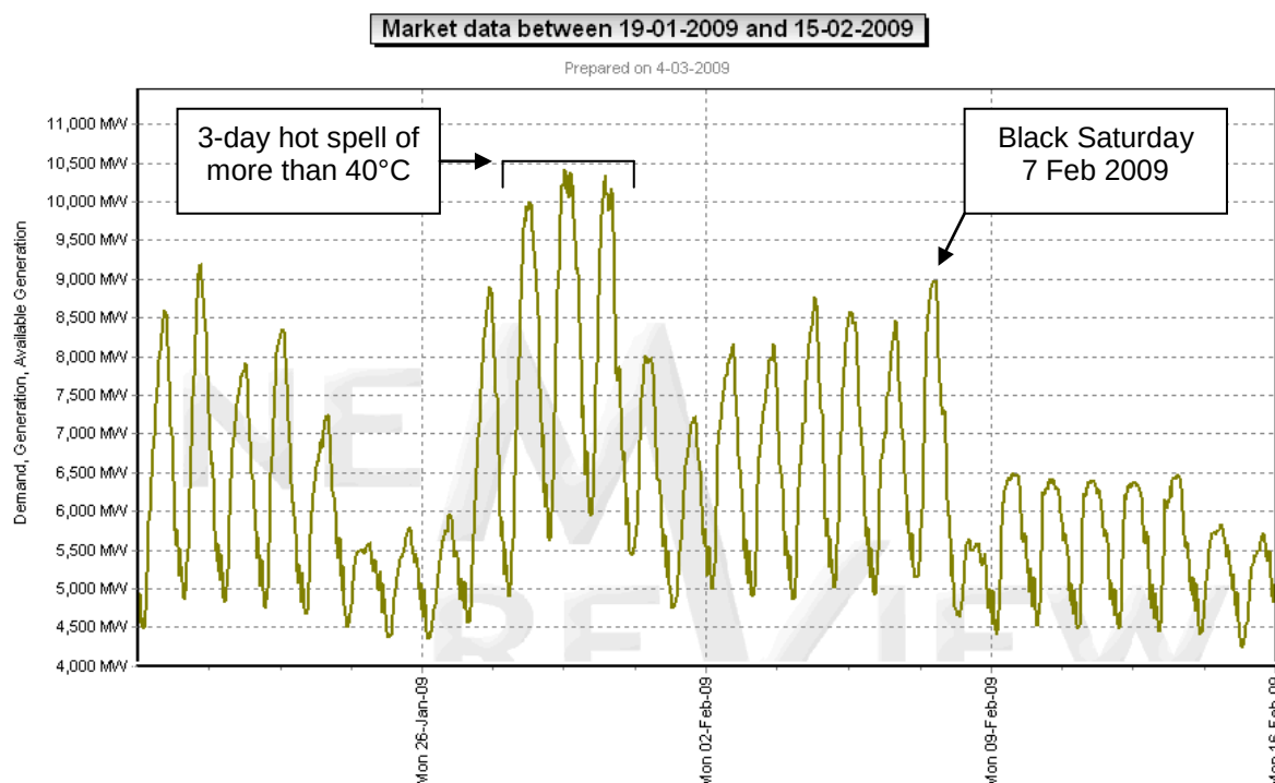
Figure 4.4: Electricity consumption of VIC from 19/01/09 to 15/02/09
