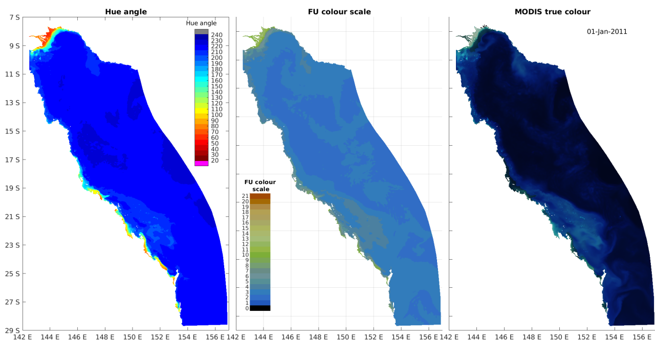
Figure 1: Simulated hue angle (left), Forel-Ule colour scale (centre) and MODIS true colour (right) calculated from simulated remote-sensing reflectance on the Great Barrier Reef on 1 Jan 2011.
