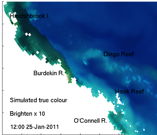
Figure 4: Observed (top) and simulated (bottom) true colour from simulated remote-sensing reflectance at 670, 555 and 470 nm in the GBR4 model configuration in the region of the Burdekin River. A brightening of 10 (left) and 20 (right) was applied for comparison.
