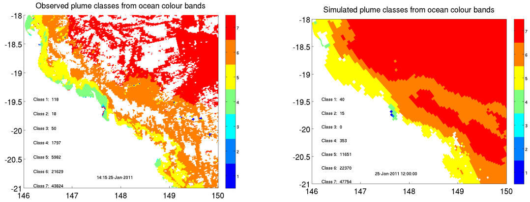
Figure 7: Observed and simulated optical plume classification on the 25 Jan 2011 in the Burdekin River region. See Fig. 6 for spectra of individual classes.
