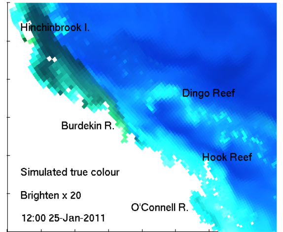
Figure 4: Observed (top) and simulated (bottom) true colour from simulated remote-sensing reflectance at 670, 555 and 470 nm in the GBR4 model configuration in the region of the Burdekin River. A brightening of 10 (left) and 20 (right) was applied for comparison.
