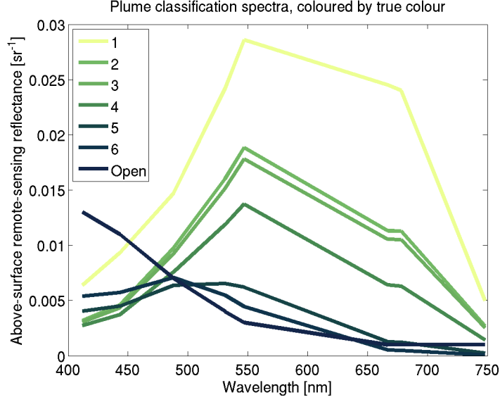
Figure 6: Spectra of each of the optical plume classifications (1-6) and the open ocean. The area in \text{km}^2 for each plume class within the region plotted is given on the left for both the observed and simulated classes.
