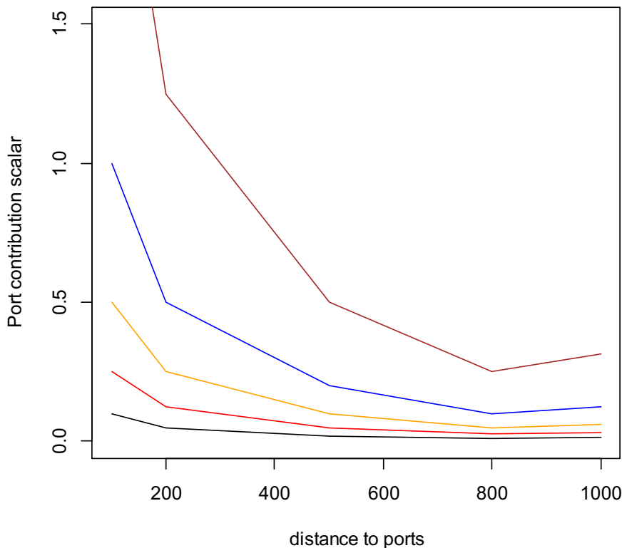
Figure 2. The port contribution scalar ( mFC/distanceZ ) for five boxes with a distance to ports set at 100, 200, 500, 800 and 1000 km (i.e. the mFCscale would be rescaled by the average distance of 520 on read-in).
